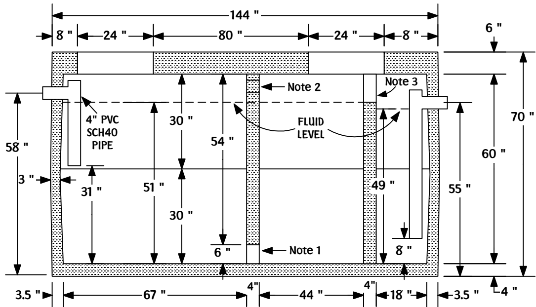
SIDE SEC.
